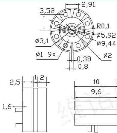
CX-A12mm-2P-M 2A 12V
