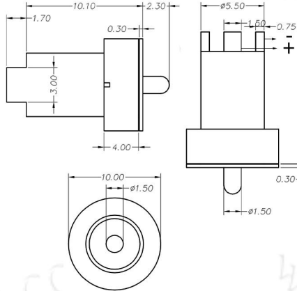
cx-902-10mm 3A 12V
