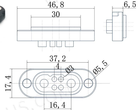
cx2+4-y4 15A 24V
