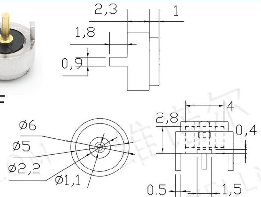
cx5-6mm-F 3A 12V
