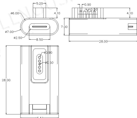
Type-c母转magsafe2
