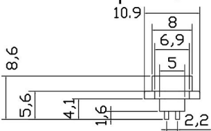
CXZ-D型-20pin公
