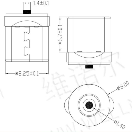
cx-Type-c plug
