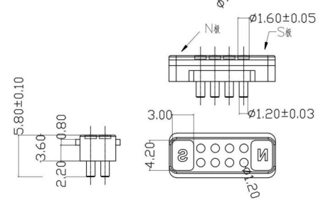
双排8p-2.0PH-02
