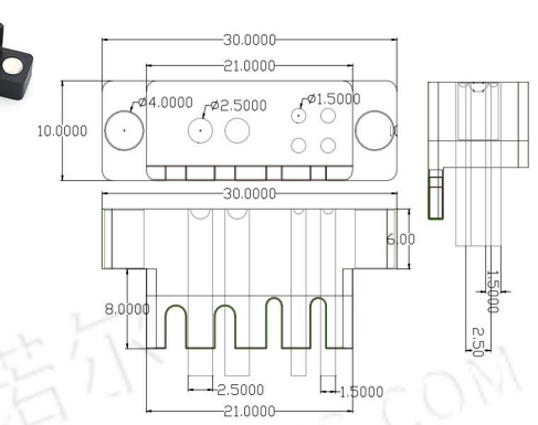
cx2+4-f2 5A 24V
