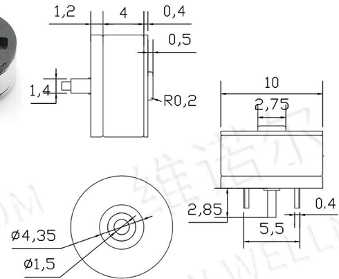
CX-XM10-F 3A 12V
