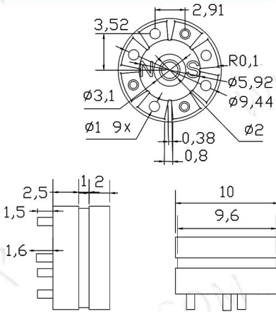
CX-A12mm-4P-M 2A 12V
