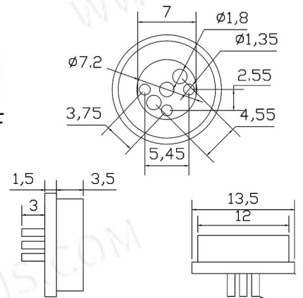
cx12-13.5mm-3P-F 2A 12V
