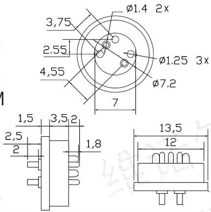
cx12-13.5mm-2P-F 2A 12V
