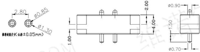
2p-2.84PH-01
