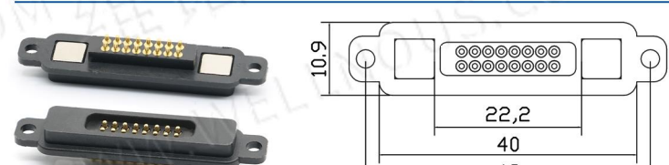
CXZ-D型-16pin公
