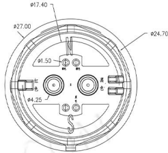
cxfs-27mmjg-m1 军工防水磁吸 18A 24V
