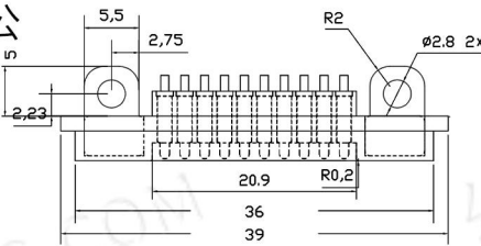
CX-FB型-20pin母
