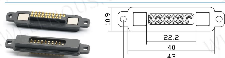
CXZ-D型-19pin公
