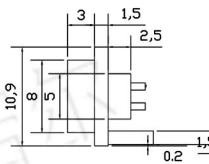
CX-FB型-20pin公
