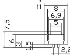
CXZ-D型-20pin母
