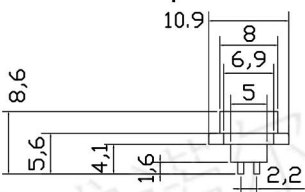
CXZ-D型-19pin公
