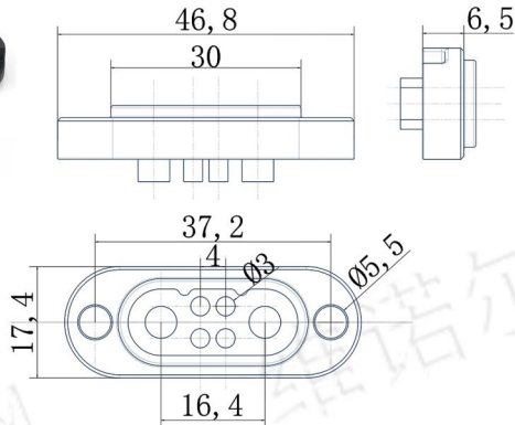
cx2+4-y1 15A 24V
