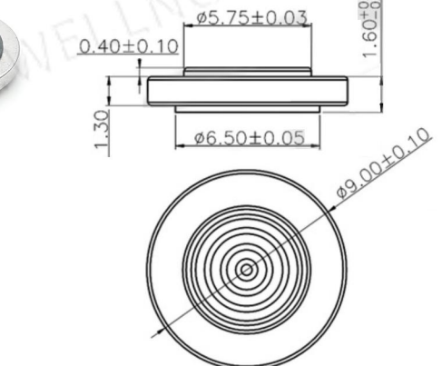
cx-9mm-7P
