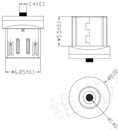
cx-Type-c plug
