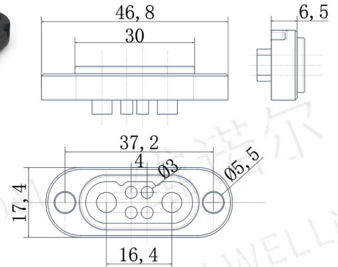
cx2+4-y2 15A 24V
